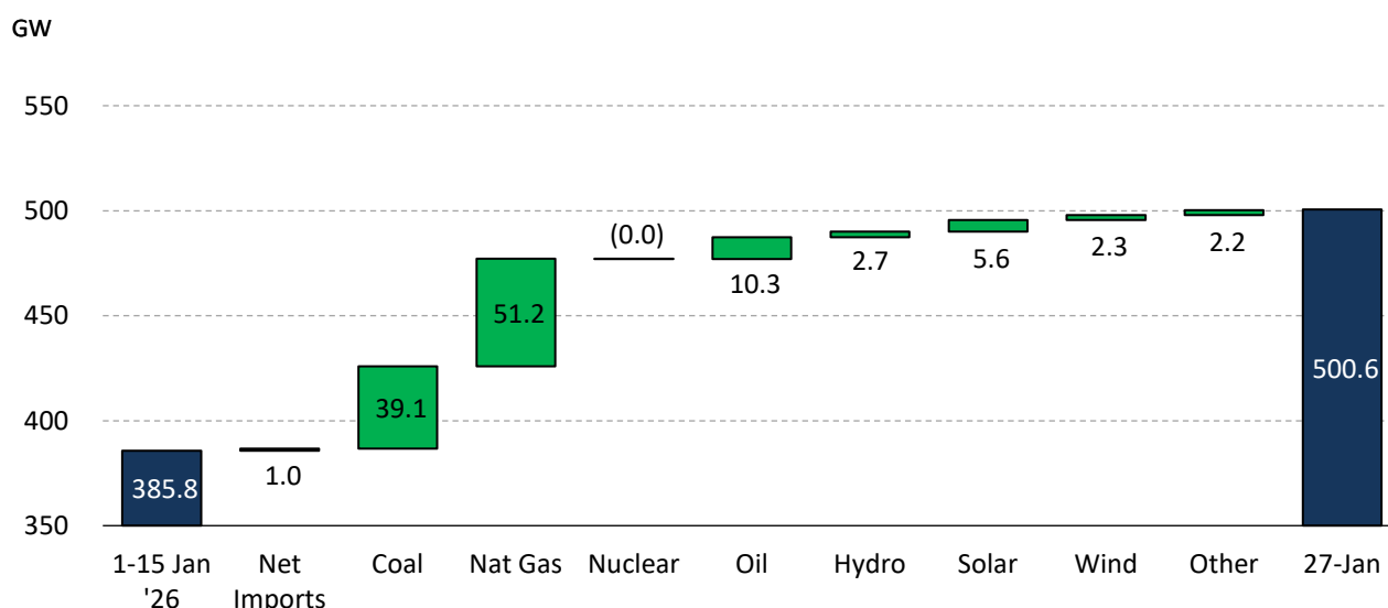
EXHIBIT 4: REGIONAL TOTAL - AVG. OPERATIONS VS. DURING PEAK DEMAND DAY OF WINTER STORM FERN
