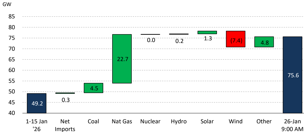
EXHIBIT 15: ERCOT - AVG. OPERATIONS VS. DURING PEAK DEMAND HOUR
