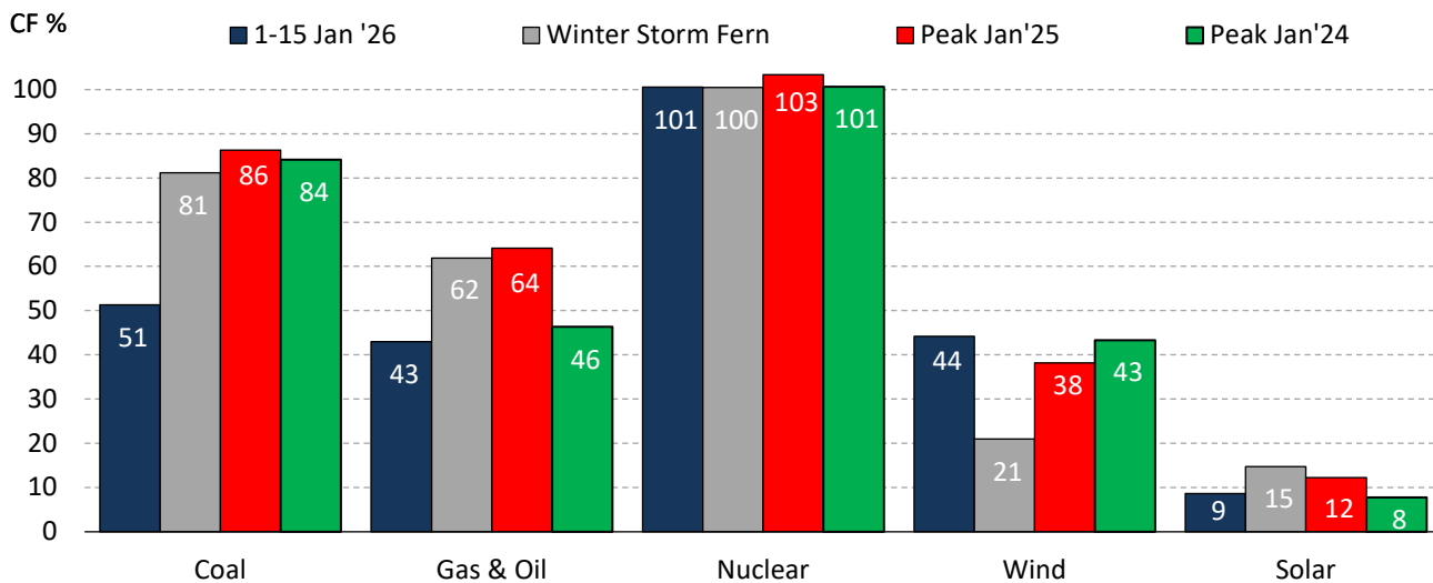
EXHIBIT 26: PJM - CAPACITY FACTOR BY FUEL TYPE DURING PEAK DEMAND TIMES
