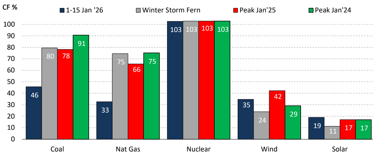
EXHIBIT 16: ERCOT - CAPACITY FACTOR BY FUEL TYPE DURING PEAK DEMAND TIMES
