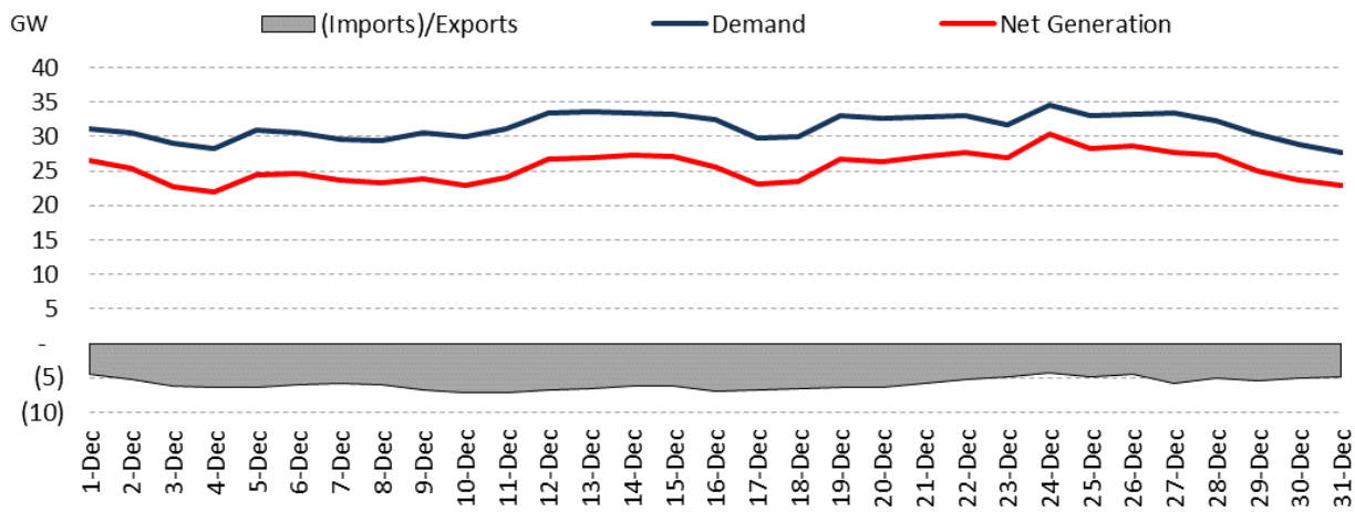
EXHIBIT 8: NORTHEAST - AVERAGE DAILY ELECTRIC DEMAND, (IMPORTS)/EXPORTS & NET GEN. – DECEMBER 2022
