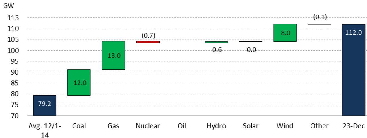
EXHIBIT 29: MISO - CHANGE IN NET GENERATION BY FUEL TYPE DURING WINTER STORM ELLIOTT
